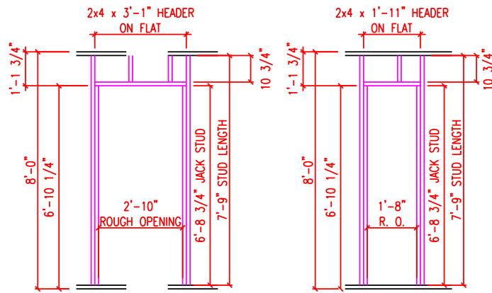
INTERIOR DOOR FRAMING
